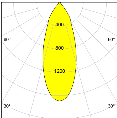
I-max : 1696 cd/klm
