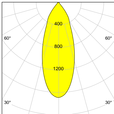
I-max : 1696 cd/klm
