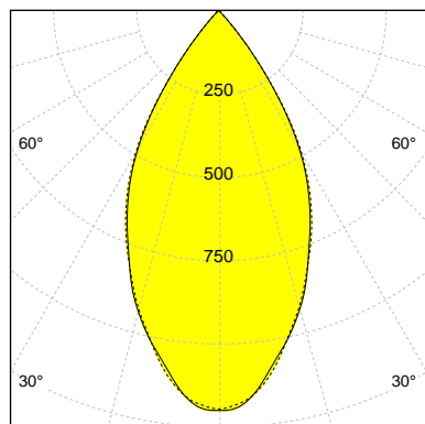
I-max : 1203 cd/klm
