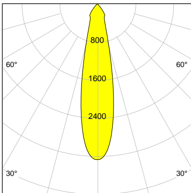
I-max : 3278 cd/klm
